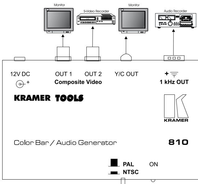
Figure 2: Connecting the 810 Color Bar / Audio Generator
